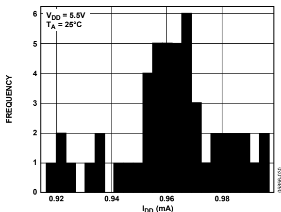
Figure 31. I_{DD} Histogram with Internal Reference, V_{REFOUT} = 2.5V
