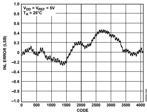
Figure 7. AD5624R INL, External Reference
