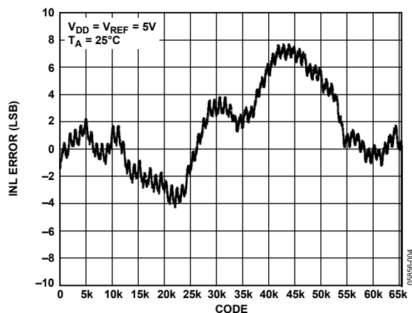
Figure 5. AD5664R INL, External Reference
