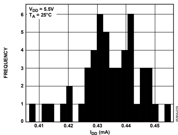
Figure 30. I_{DD} Histogram with External Reference, 5.5 V
