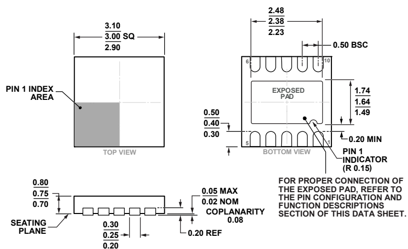
Figure 65. 10-Lead Lead Frame Chip Scale Package [LFCSP_WD] 3 mm × 3 mm Body, Very Very Thin, Dual Lead (CP-10-9)
