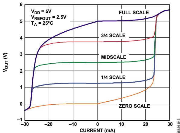
Figure 35. AD56x4R-5 Source and Sink Capability
