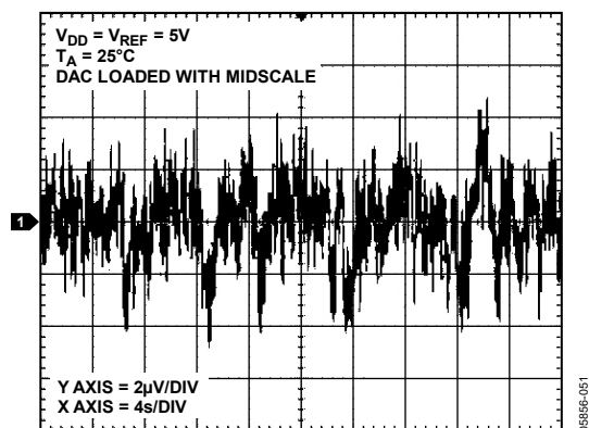
Figure 44. 0.1 Hz to 10 Hz Output Noise Plot, External Reference
