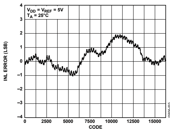
Figure 6. AD5644R INL, External Reference
